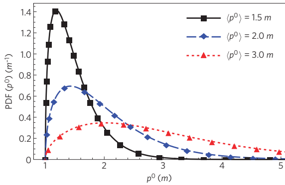
Figure 2 | Equilibrium energy distribution of relativistic gas particles in the lab frame. Our numerical results (symbols) are in good agreement with the theoretically expected Jüttner distribution (lines) from equation (3b) for various values of the mean particle energy ( p^0 ), which confirms the adequacy of the algorithm used (see the Methods section).
