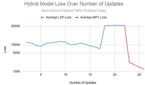
Figure 4: Hybrid Model Loss Over Number of Updates. Semi-Honest Shamir MPC Protocol was Used
