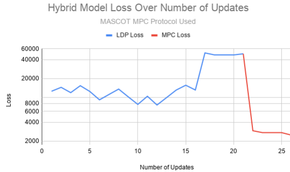
Figure 2: Hybrid Model Loss Over Number of Updates. MASCOT MPC Protocol was Used
