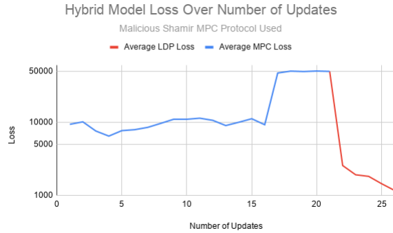
Figure 6: Hybrid Model Loss Over Number of Updates. Malicious Shamir MPC was Used
