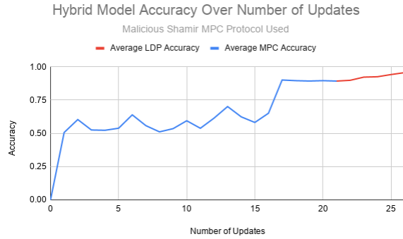
Figure 5: Hybrid Model Accuracy Over Number of Updates. Malicious Shamir MPC Protocol was Used
