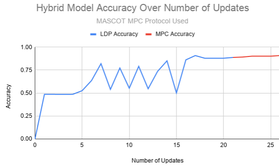
Figure 1: Hybrid Model Accuracy Over Number of Updates. MASCOT MPC Protocol was Used
