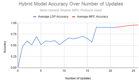
Figure 3: Hybrid Model Accuracy Over Number of Updates. Semi-Honest Shamir MPC Protocol was Used
